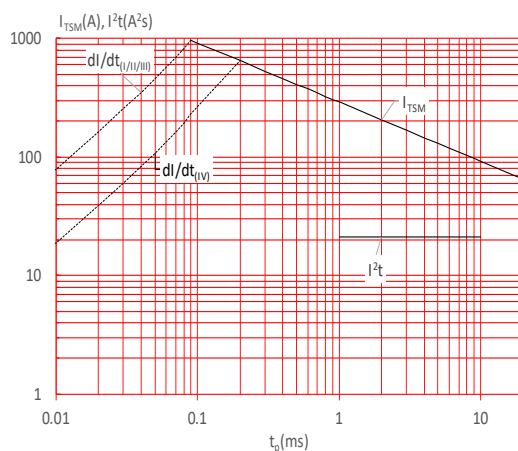
FIG.6: Non-repetitive surge peak on-state current for a sinusoidal pulse with width t_p < 20ms , and corresponding value of I^2t ( I - II - III: di/dt < 50A/\mu s ; IV: di/dt < 20A/\mu s )
