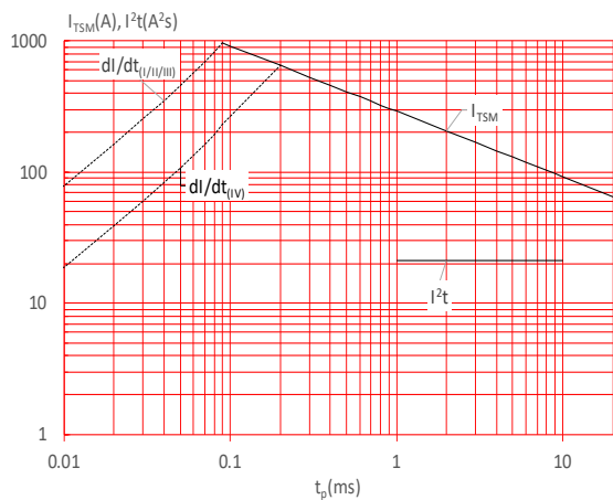
FIG.5: Non-repetitive surge peak on-state current for a sinusoidal pulse with width t_p < 20\text{ms} , and corresponding value of I^2t (I - II - III: dl/dt < 100\text{A}/\mu\text{s} ; IV: dl/dt < 50\text{A}/\mu\text{s} )
