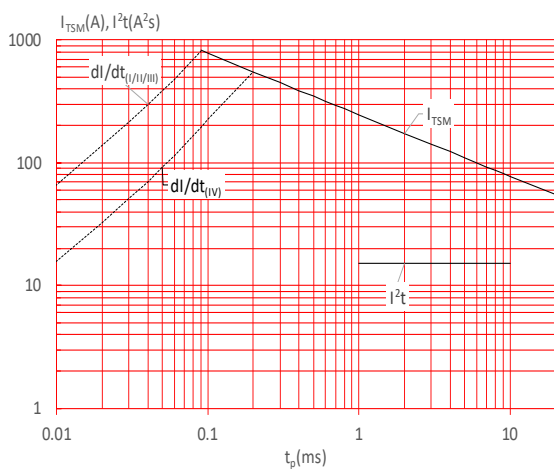
FIG.5: Non-repetitive surge peak on-state current for a sinusoidal pulse with width t_p < 20ms , and corresponding value of I^2t (I - II - III: dl/dt < 70A/\mu s ; IV: dl/dt < 40A/\mu s )
