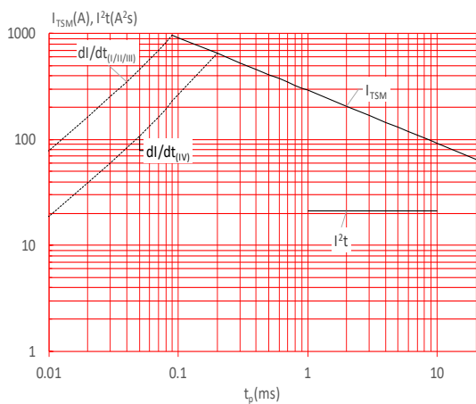
FIG.5: Non-repetitive surge peak on-state current for a sinusoidal pulse with width t_p < 20\text{ms} , and corresponding value of I^2t (I - II - III: dl/dt < 80\text{A}/\mu\text{s} ; IV: dl/dt < 40\text{A}/\mu\text{s} )
