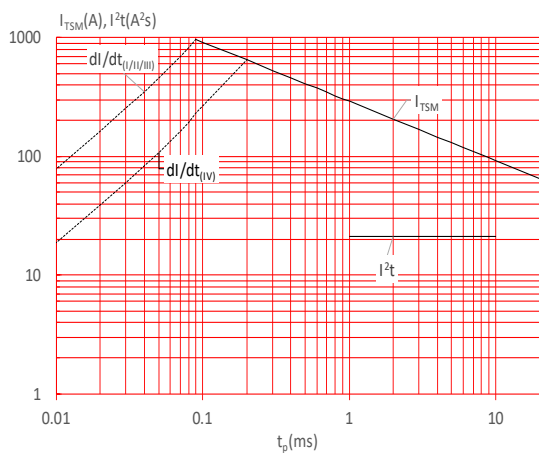
FIG.5: Non-repetitive surge peak on-state current for a sinusoidal pulse with width t_p < 20\text{ms} , and corresponding value of I^2t (I - II - III: dl/dt < 100\text{A}/\mu\text{s} ; IV: dl/dt < 50\text{A}/\mu\text{s} )
