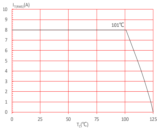
FIG.4: On-state characteristics
