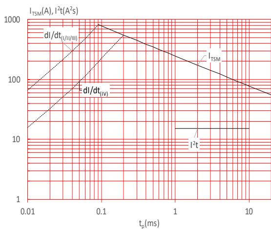
FIG.5: Non-repetitive surge peak on-state current for a sinusoidal pulse with width t_p < 20\text{ms} , and corresponding value of I^2t (I - II - III: dl/dt < 70\text{A}/\mu\text{s} ; IV: dl/dt < 40\text{A}/\mu\text{s} )
