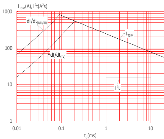
FIG.5: Non-repetitive surge peak on-state current for a sinusoidal pulse with width t_p < 20\text{ms} , and corresponding value of I^2t (I - II - III: dl/dt < 50\text{A}/\mu\text{s} ; IV: dl/dt < 30\text{A}/\mu\text{s} )
