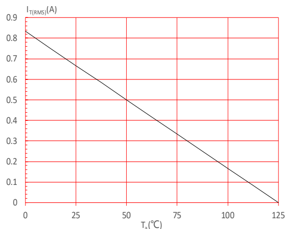
FIG.5: On-state characteristics
