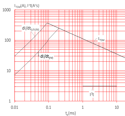
FIG.6: Non-repetitive surge peak on-state current for a sinusoidal pulse with width t_p < 20ms , and corresponding value of I^2t (I - II - III: di/dt < 50A/\mu s ; IV: di/dt < 40A/\mu s )
