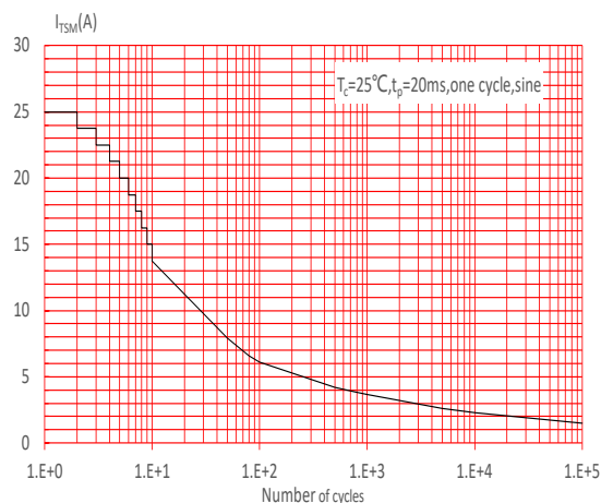
FIG.6: Non-repetitive surge peak on-state current for a sinusoidal pulse with width t_p < 20ms , and corresponding value of I^2t (I - II: di/dt < 50A/\mu s ; III-IV: di/dt < 30A/\mu s )
