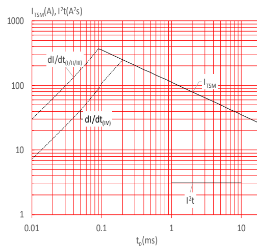
FIG.6: Non-repetitive surge peak on-state current for a sinusoidal pulse with width t_p < 20ms , and corresponding value of I^2t (I - II - III: di/dt < 80A/\mu s ; IV: di/dt < 40A/\mu s )
