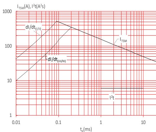
FIG.5: Non-repetitive surge peak on-state current for a sinusoidal pulse with width t_p < 20\text{ms} , and corresponding value of I^2t ( I - II: di/dt < 50\text{A}/\mu\text{s}; III - IV: di/dt < 30\text{A}/\mu\text{s} )
