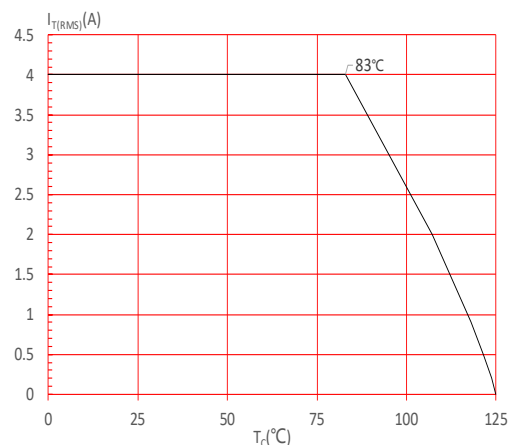
FIG.4: On-state characteristics
