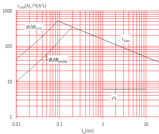
FIG.5: Non-repetitive surge peak on-state current for a sinusoidal pulse with width t_p < 20\text{ms} , and corresponding value of I^2t ( I - II: dl/dt < 50\text{A}/\mu\text{s}; III-IV: dl/dt < 30\text{A}/\mu\text{s} )
