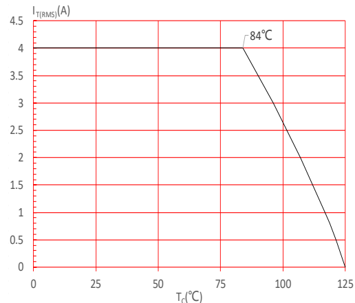
FIG.4: On-state characteristics
