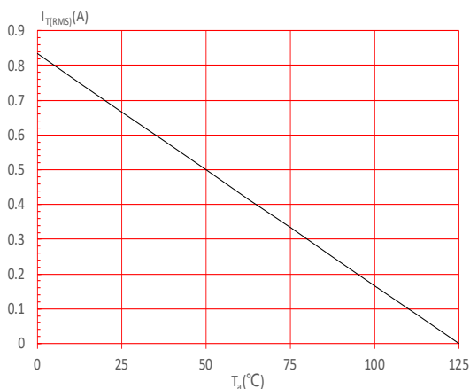
FIG.5: On-state characteristics
