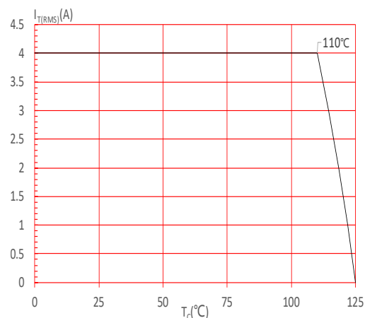
FIG.4: On-state characteristics
