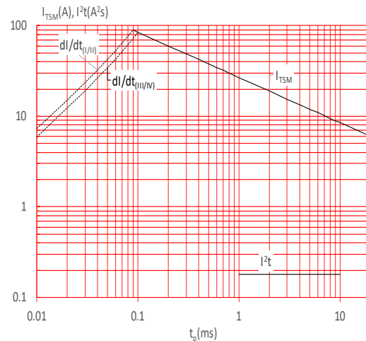
FIG.6: Non-repetitive surge peak on-state current for a sinusoidal pulse with width t_p < 20\text{ms} , and corresponding value of I^2t (I - II: di/dt < 50\text{A}/\mu\text{s} ; III-IV: di/dt < 20\text{A}/\mu\text{s} )
