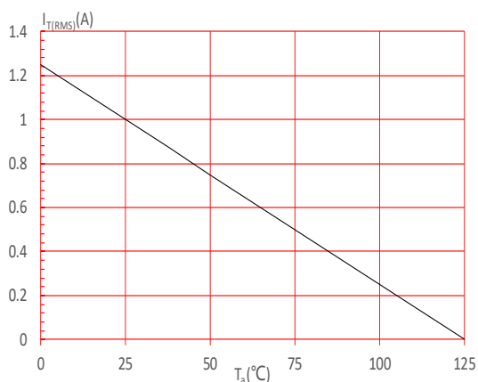
FIG.5: On-state characteristics
