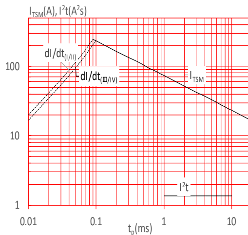
FIG.6: Non-repetitive surge peak on-state current for a sinusoidal pulse with width t_p < 20ms , and corresponding value of I^2t ( I - II: di/dt < 30A/\mu s ; III-IV: di/dt < 20A/\mu s )
