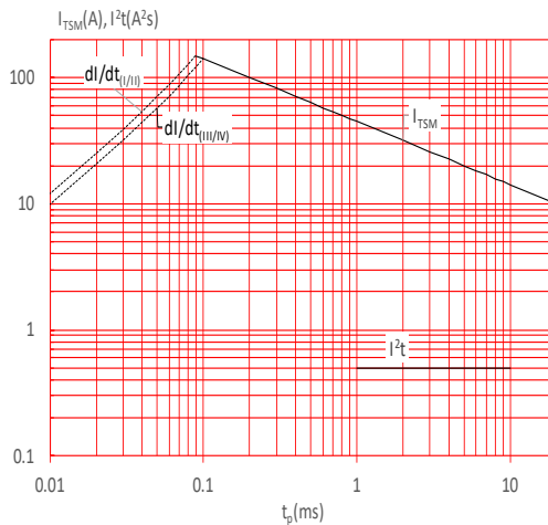
FIG.6: Non-repetitive surge peak on-state current for a sinusoidal pulse with width t_p < 20\text{ms} , and corresponding value of I^2t ( I - II: dI/dt < 30\text{A}/\mu\text{s} ; III-IV: dI/dt < 20\text{A}/\mu\text{s} )
