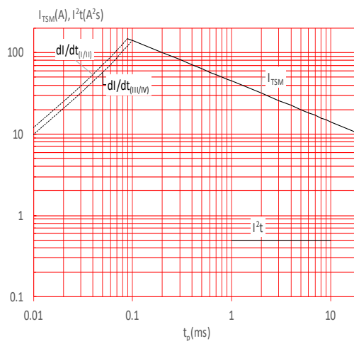
FIG.6: Non-repetitive surge peak on-state current for a sinusoidal pulse with width t_p < 20ms , and corresponding value of I^2t ( I - II: di/dt < 50A/\mu s ; III-IV: di/dt < 30A/\mu s )
