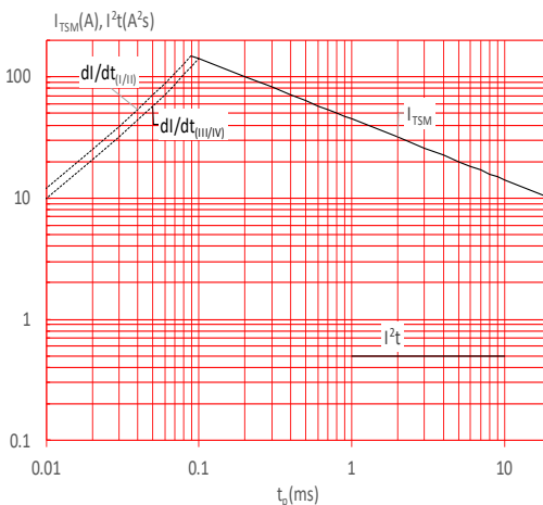
FIG.6: Non-repetitive surge peak on-state current for a sinusoidal pulse with width t_p < 20ms , and corresponding value of I^2t (I - II : di/dt < 50A/μs ; III-IV : di/dt < 30A/μs )
