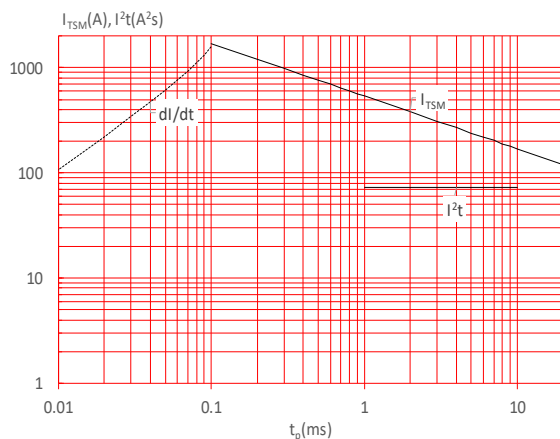
FIG.5: Non-repetitive surge peak on-state current for a sinusoidal pulse with width t_p < 20ms , and corresponding value of I^2t ( dl/dt < 100A/\mu s )
