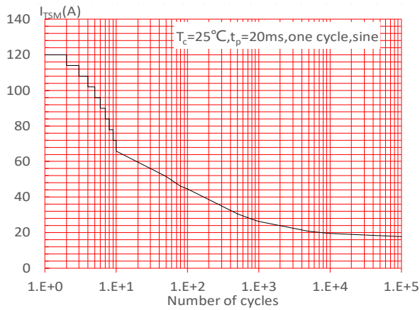
FIG.5: Non-repetitive surge peak on-state current for a sinusoidal pulse with width t_p < 20ms , and corresponding value of I^2t ( dl/dt < 100A/\mu s )
