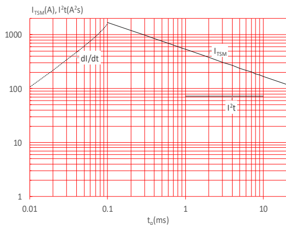
FIG.5: Non-repetitive surge peak on-state current for a sinusoidal pulse with width t_p < 20ms , and corresponding value of I^2t ( dl/dt < 50A/\mu s )
