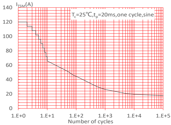
FIG.5: Non-repetitive surge peak on-state current for a sinusoidal pulse with width t_p < 20ms , and corresponding value of I^2t ( dl/dt < 50A/\mu s )
