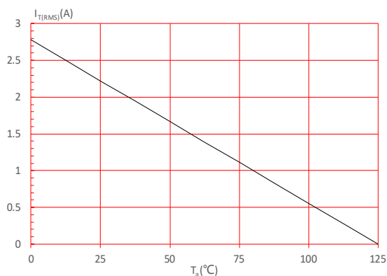
FIG.5: On-state characteristics
