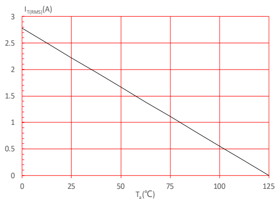
FIG.5: On-state characteristics
