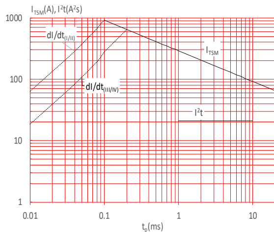
FIG.5: Non-repetitive surge peak on-state current for a sinusoidal pulse with width t_p < 20ms , and corresponding value of I^2t ( I - II : dl/dt < 100A/\mu s ; III-IV : dl/dt < 50A/\mu s )
