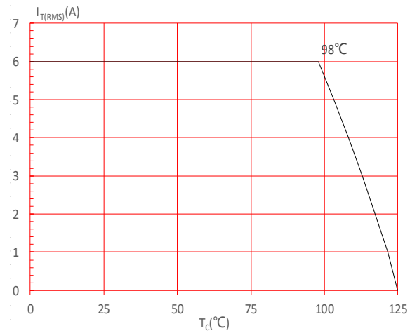
FIG.4: On-state characteristics
