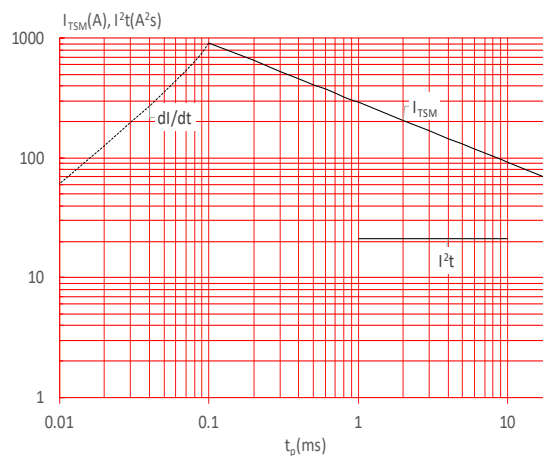
FIG.6: Non-repetitive surge peak on-state current for a sinusoidal pulse with width t_p < 20ms , and corresponding value of I^2t ( dl/dt < 100A/\mu s )
