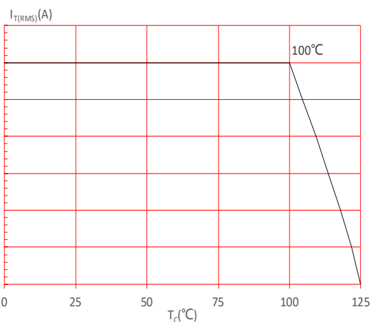
FIG.4: On-state characteristics
