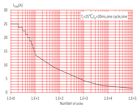
FIG.6: Non-repetitive surge peak on-state current for a sinusoidal pulse with width t_p < 20ms , and corresponding value of I^2t ( di/dt < 50A/μs )
