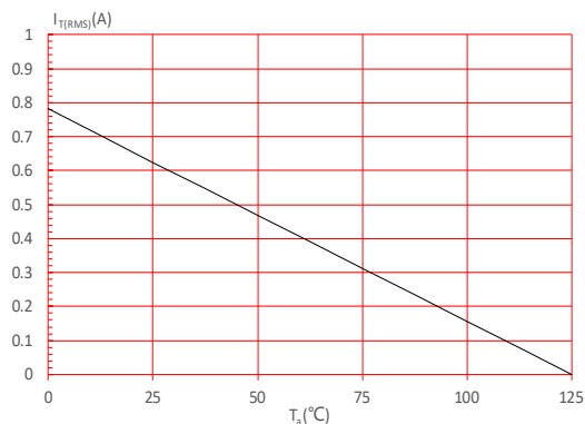
FIG.5: On-state characteristics
