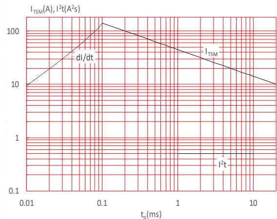
FIG.5: Non-repetitive surge peak on-state current for a sinusoidal pulse with width t_p < 20ms , and corresponding value of I^2t ( dl/dt < 80A/\mu s )
