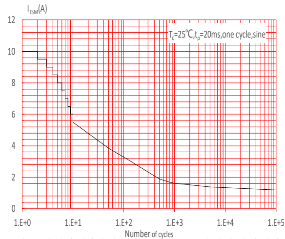
FIG.5: Non-repetitive surge peak on-state current for a sinusoidal pulse with width t_p < 20ms , and corresponding value of I^2t ( dl/dt < 80A/\mu s )
