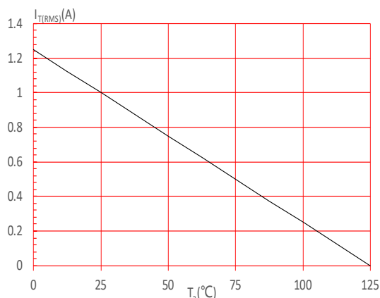
FIG.5: On-state characteristics
