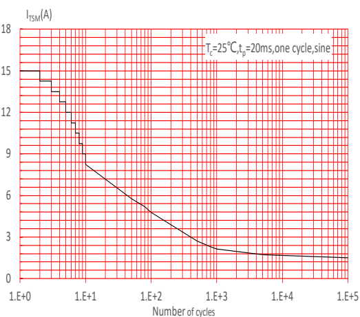
FIG.6: Non-repetitive surge peak on-state current for a sinusoidal pulse with width t_p < 20ms , and corresponding value of I^2t ( dl/dt < 60A/\mu s )
