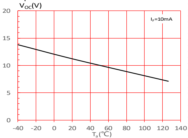
FIG.5: Open Circuit Voltage vs. Ambient Temperature
