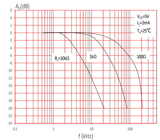
FIG.10: Frequency Response
