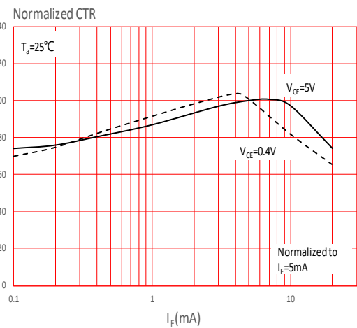
FIG.6: Normalized Current Transfer Ratio vs. Forward Current
