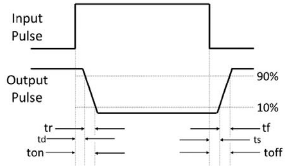
FIG.12: Curves of Response Time
