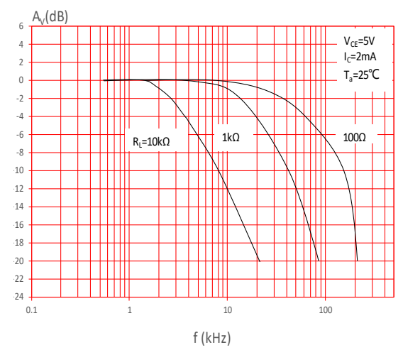
FIG.10: Frequency Response
