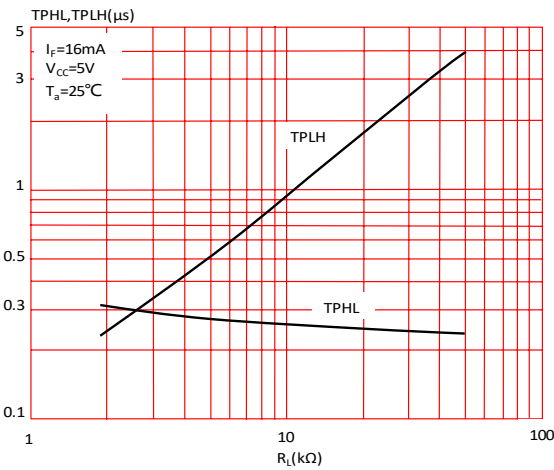
FIG.8: Propagation Delay vs. Load Resistance
