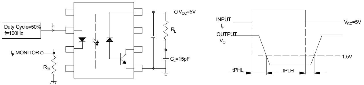
Fig.10: Test Circuit of tPHL, tPLH
