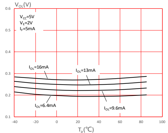
FIG.6: Low Level Output Voltage vs. Ambient Temperature
