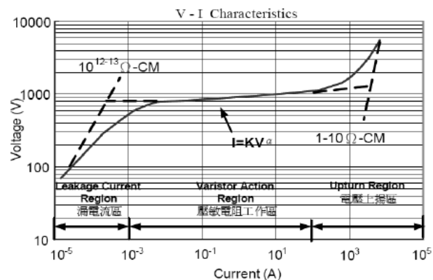
Varistor V-I characteristics curve
