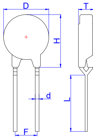
Y Lead Type (Y Kink Lead)
