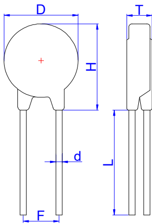
P Type (Straight Lead)
