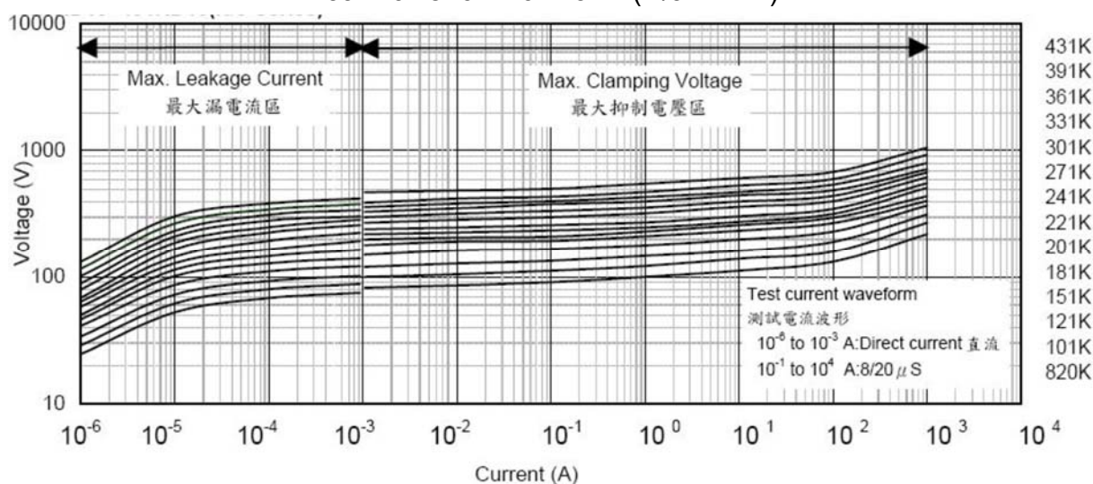
JJV10D820K-10D431K (N/J series)
