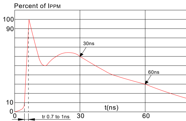
FIG.4: ESD clamping (25kV contact)
